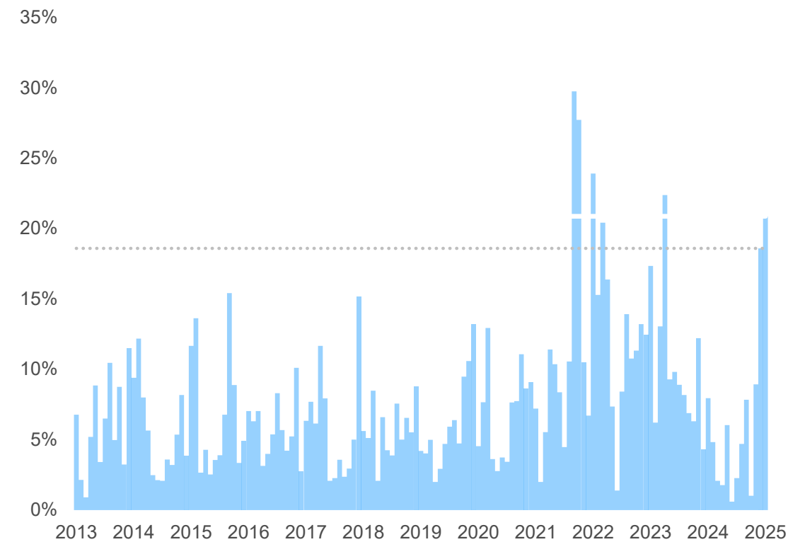
Monthly urea volatility (US FOB NOLA)
